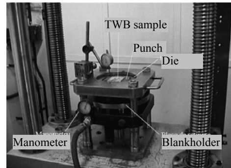
Figure 3. Experimental device
