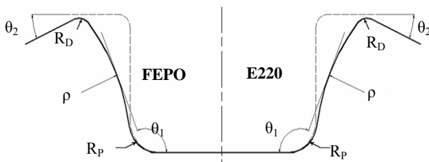
Figure 2. Springback parameters
