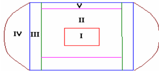
Figure 4. Deformation zones on round samples
