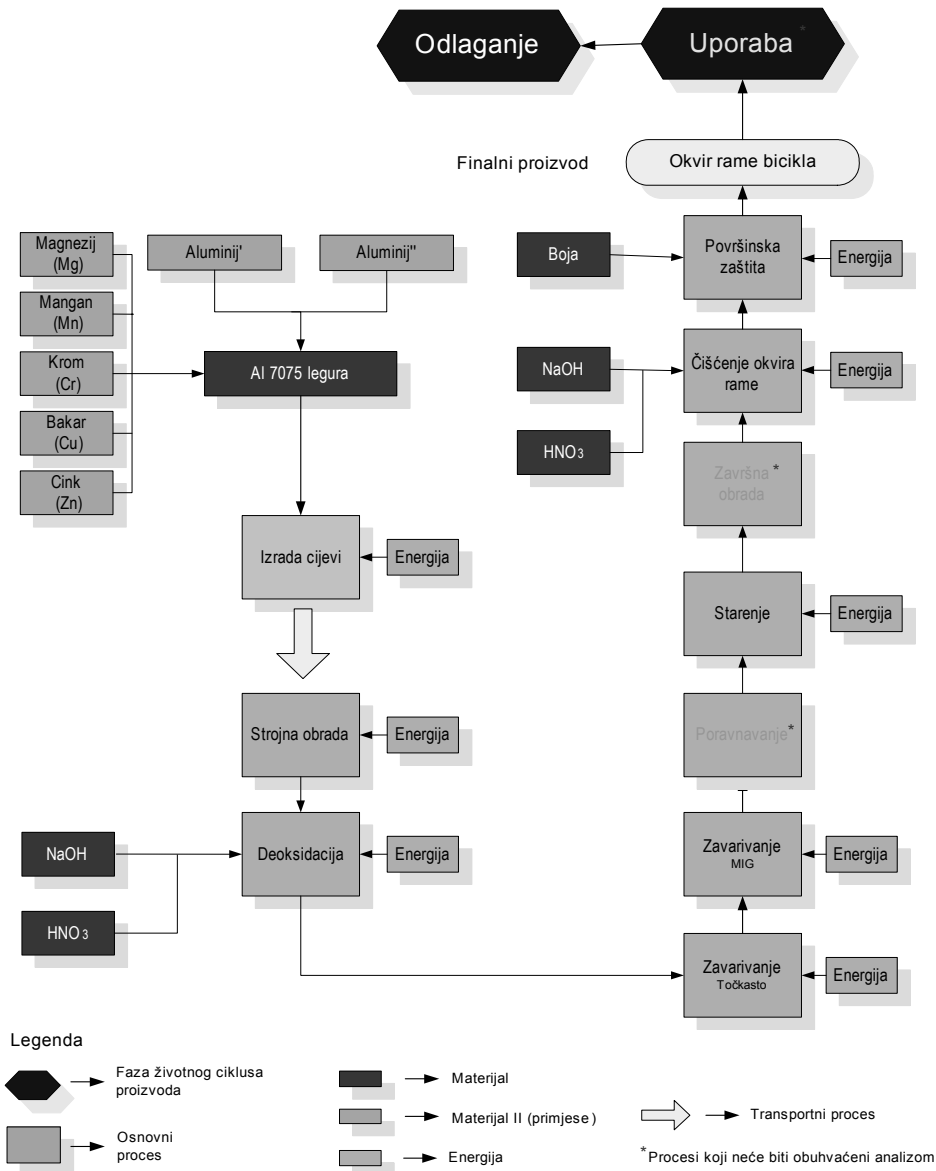
Figure 1. Estimation of influence potentials for some environmental emissions of case study [8]
