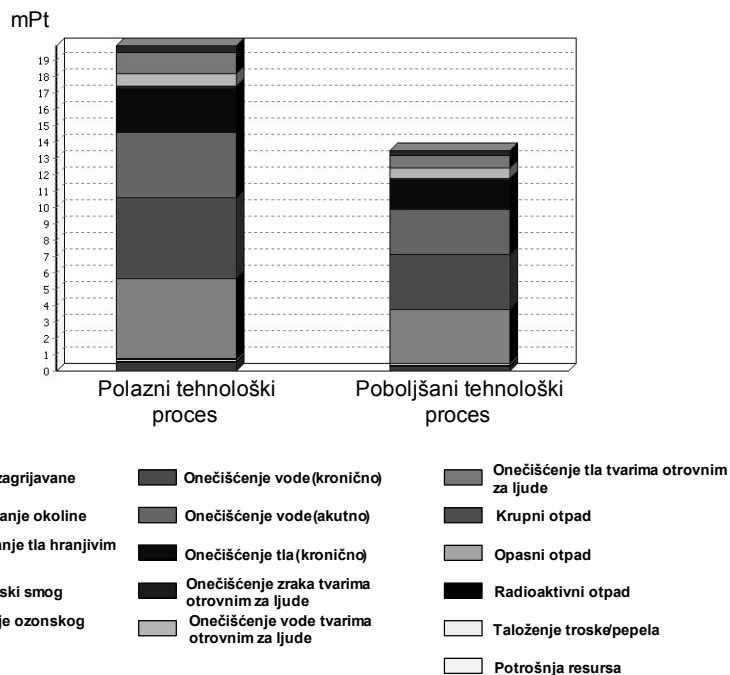
Figure 5. Comparison of the initial and improved technological processes [8]
