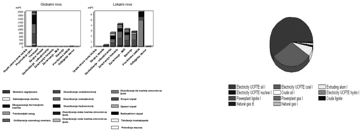
Figure 4. Portion of total environmental contamination some subprocesses in observed process of Al alloy extrusion [8]
