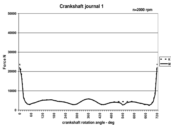
Figure 3 Crankshaft Journals 1
