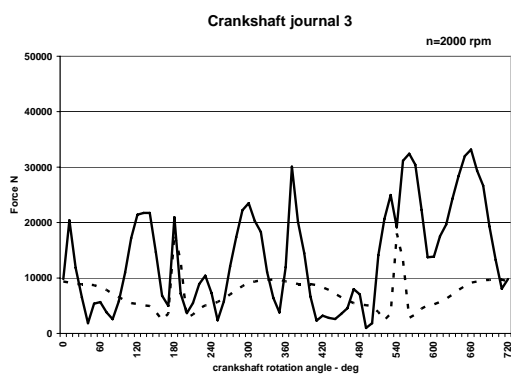
Figure 6 Crankshaft Journals 4
