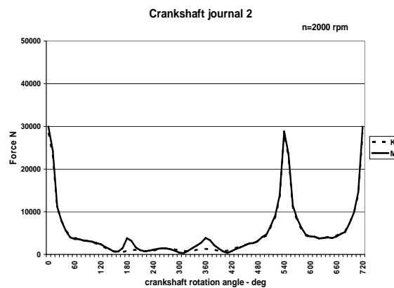
Figure 4 Crankshaft Journals 2
