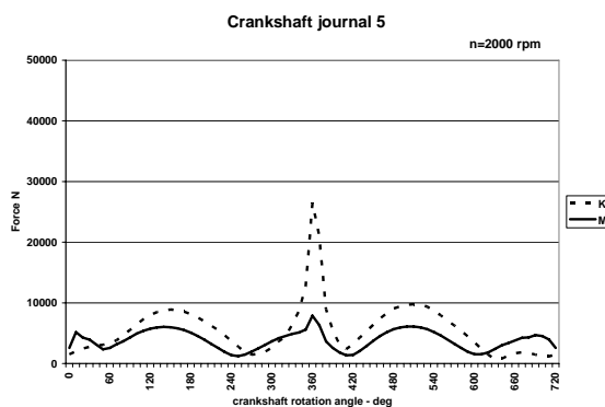
Figure 7 Crankshaft Journals 5
