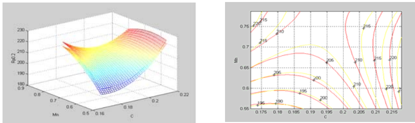
Figure 7. The delimitation of the best field for the technical running limit R_{p0,2/450} , depending on the carbon and manganese content, taking into consideration the medium percentage of silicium
