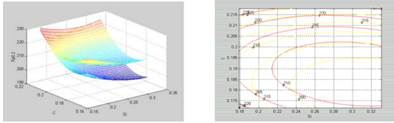
Figure 6. The delimitation of the best field for the technical running limit R_{p0,2/450} , depending on the carbon and silicium content, taking into consideration the medium percentage of manganese
