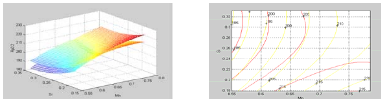
Figure 5. The delimitation of the best field for the technical running limit R_{p0,2/450} , depending on the manganese and silicium content, taking into consideration the medium percentage of carbon
