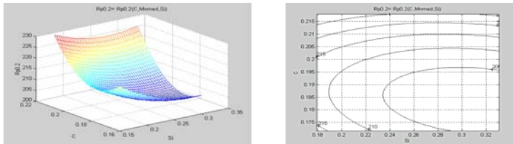
Figure 3. The variation of the technical running limit R_{p0,2/450} , containing carbon and silicium, taking into consideration the medium percentage of manganese
