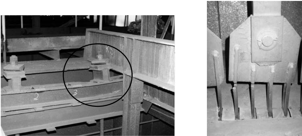
Figure 4. Grate deformation and fracture of suspension pins after overloading.
