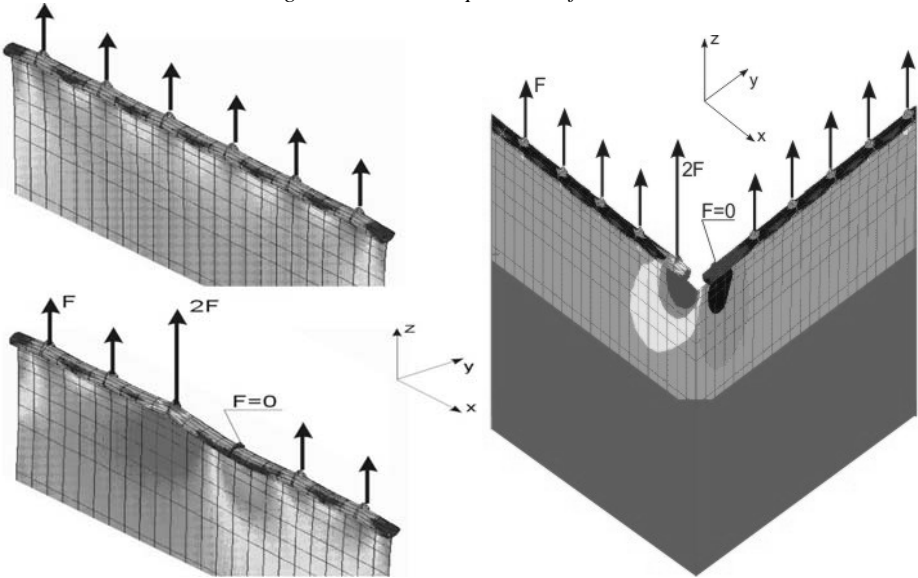
Figure 1. Elastic suspensions of boiler.
