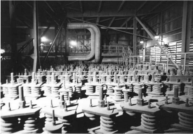
Figure 1. Elastic suspensions of boiler.
