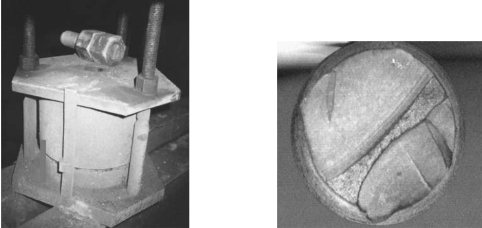
Figure 3. Fatigue failure of the suspension caused by vibrations.
