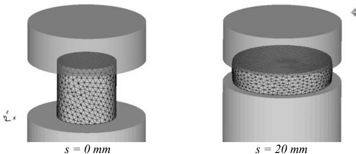
Figure 4. FE simulation in Simufact Forming 10.0
