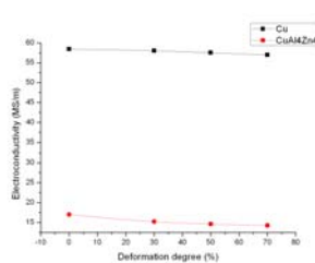
Figure 2. Dependence of electrical conductivity of cold rolled samples on deformation degree
