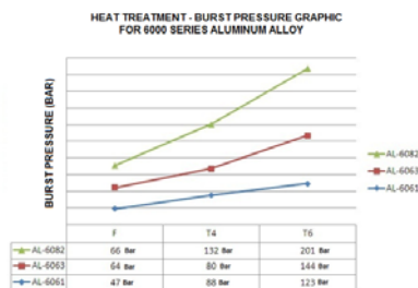
Figure 3. Hydrostatic test results
