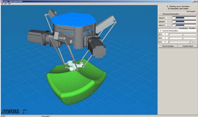
Figure 3. Analysis of robot workspace
