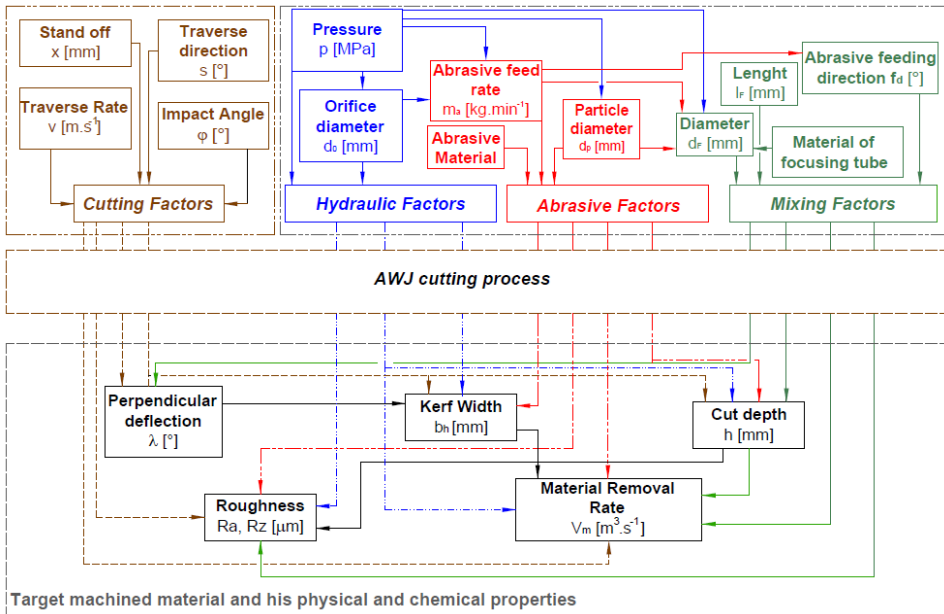
Figure 1. AWJM process model, factors vs. response parameters [4]
