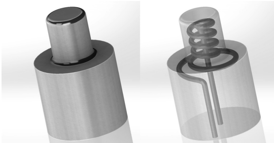
Figure 1. Tool insert with conformal cooling channel
