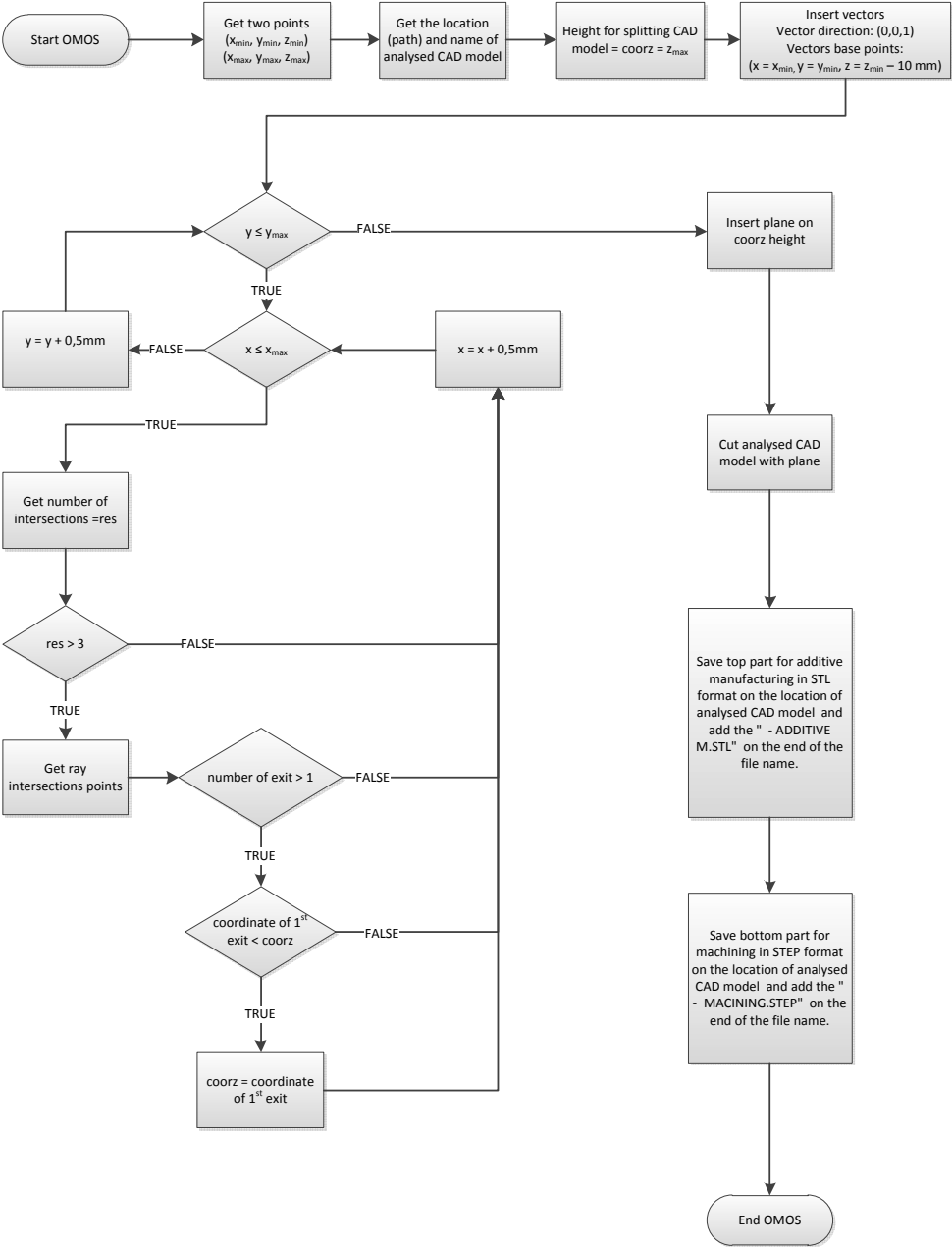
Figure 3. Flowchart of algorithm for CAD model analysis
