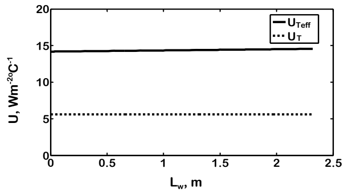
Figure 3. The effect of the latent heat in waste gas on total heat transfer coefficient of compact heat exchanger
