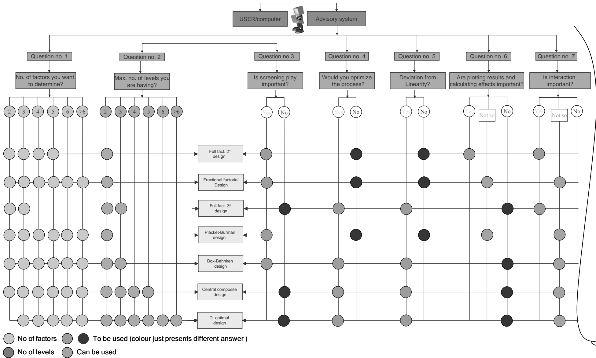
Figure 2. Schema of questions rules and definitions in web advisory system (shortened) [5]
