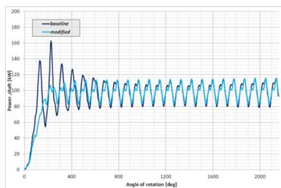
Figure 4. Power required by the compressor shaft
