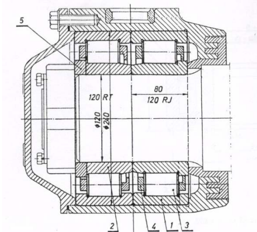
Figure 1. Switching drawing bearing with lubricator
