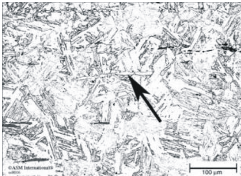
Figure 2. Microstructure of 17-7 PH steels Vilela reagent, x1000 [8].
