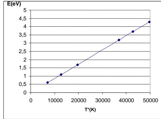
Figure 4. The dependence of the activation energy on the hopping temperature
