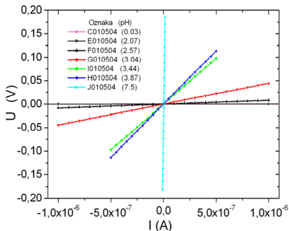
Figure 2. Current-voltage characteristics of polyaniline samples
