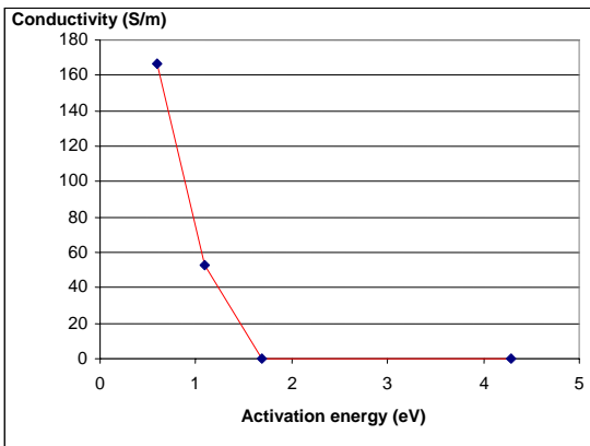
Figure 7. The dependence of the conductivity on activation energy.
