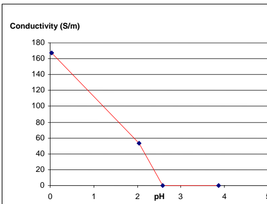
Figure 5. The dependence of the conductivity on pH values
