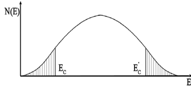
Figure 8. Density of states in disordered systems
