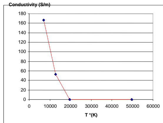
Figure 6. The dependence of the conductivity on the hopping temperature
