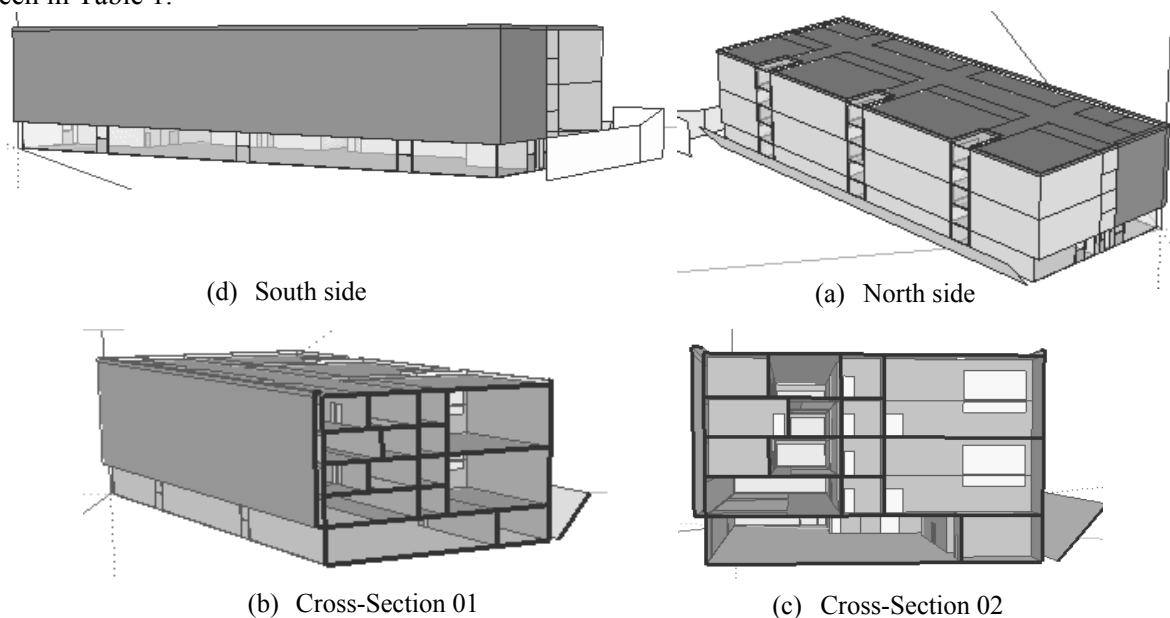
Figure 1. Energy-plus geometry of Ayazağa Central Classrooms Building
