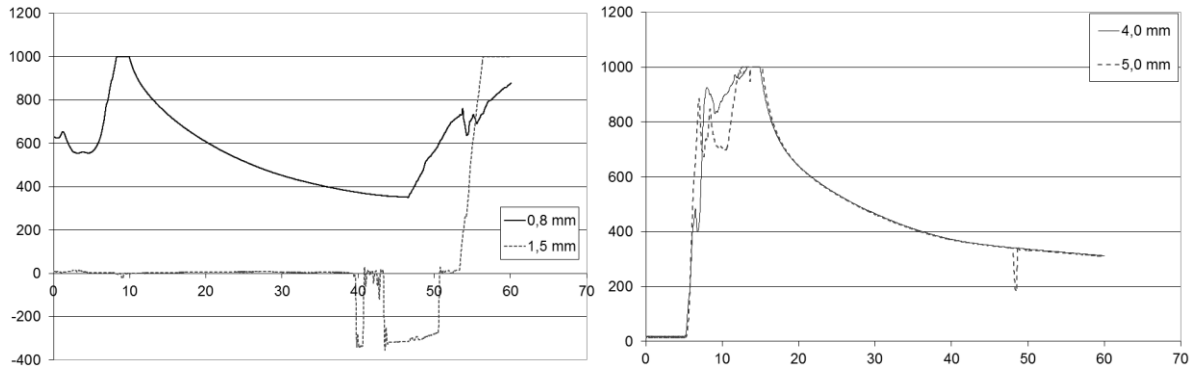
Figure 5. Temperatures measured during welding at different distances from contact surface
