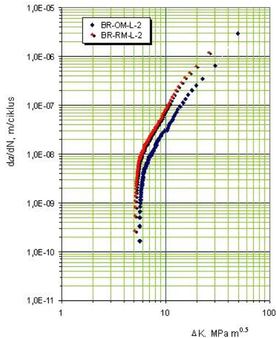
Figure 3. Relation da/dN-\Delta K for specimens in new and used materials, tested at room temperature
