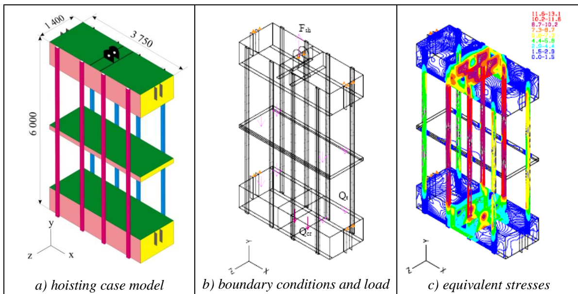
Figure 1. Hoisting cage model and structural analysis
