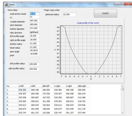
Fig. Axial section of the worm ( r_f = 2.5 [mm])
