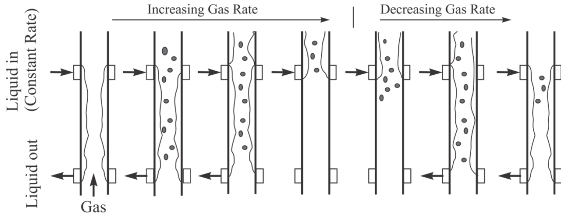
Figure 1 The processes of flooding (left) and flow reversal (right) in a vertical pipe in which liquid injection takes place via a porous segment of the pipe (adapted from [2]).
