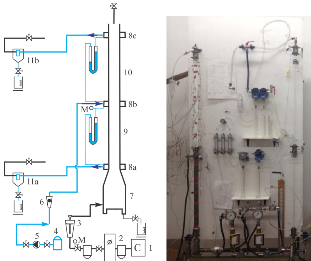
Figure 2 Experimental set-up: a) line diagram and b) a photograph view.
