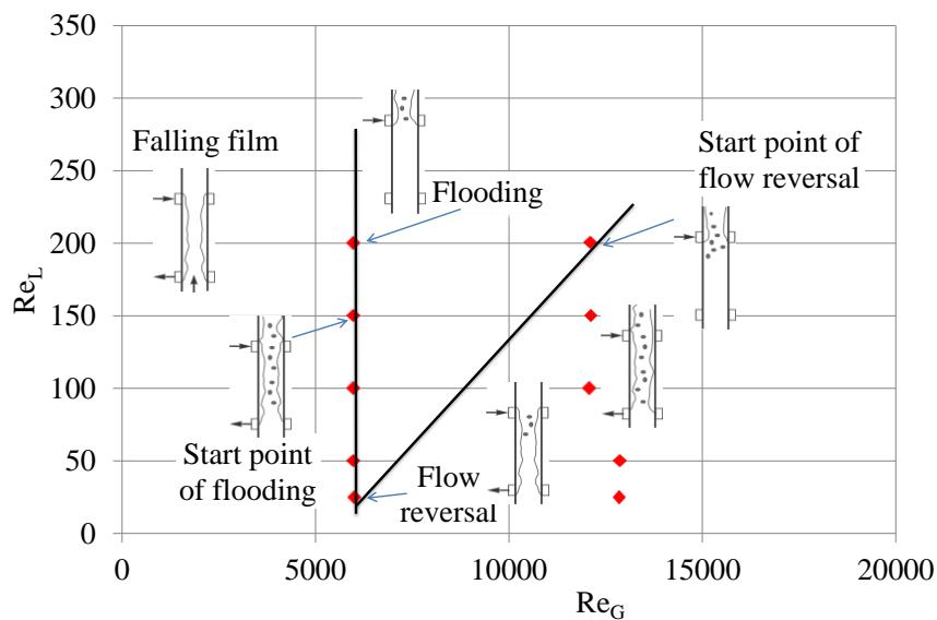
Figure 3 Ratio of Reynolds numbers for the air and the water at a constant flow of air.
